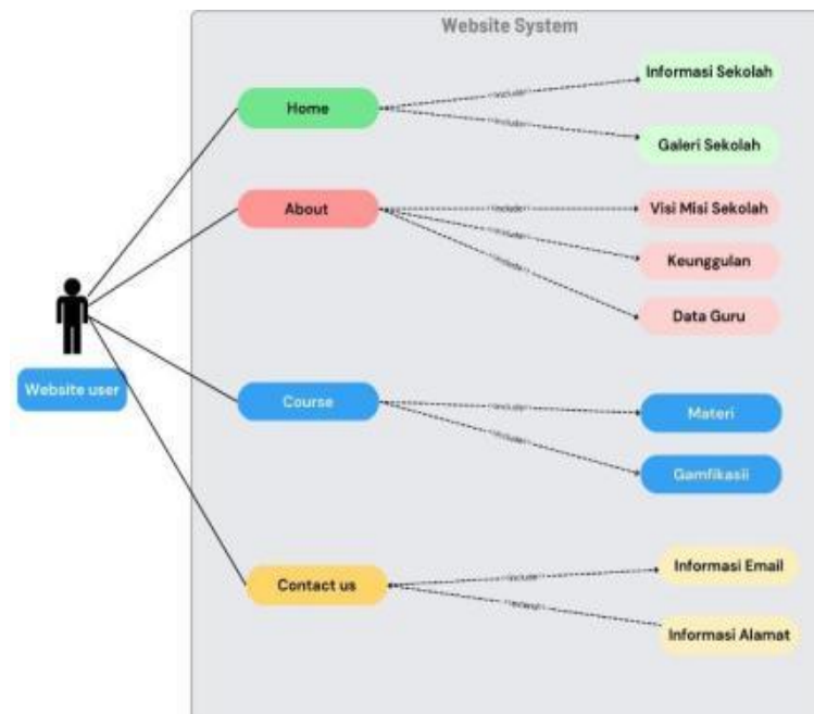
Gambar 1. Diagram Use
